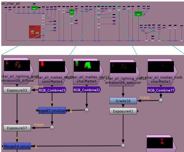
Fig. 16. Compositing graph of just the character layer of Figure 15, showing the dozens of render outputs the artist uses to assemble the final frame.
