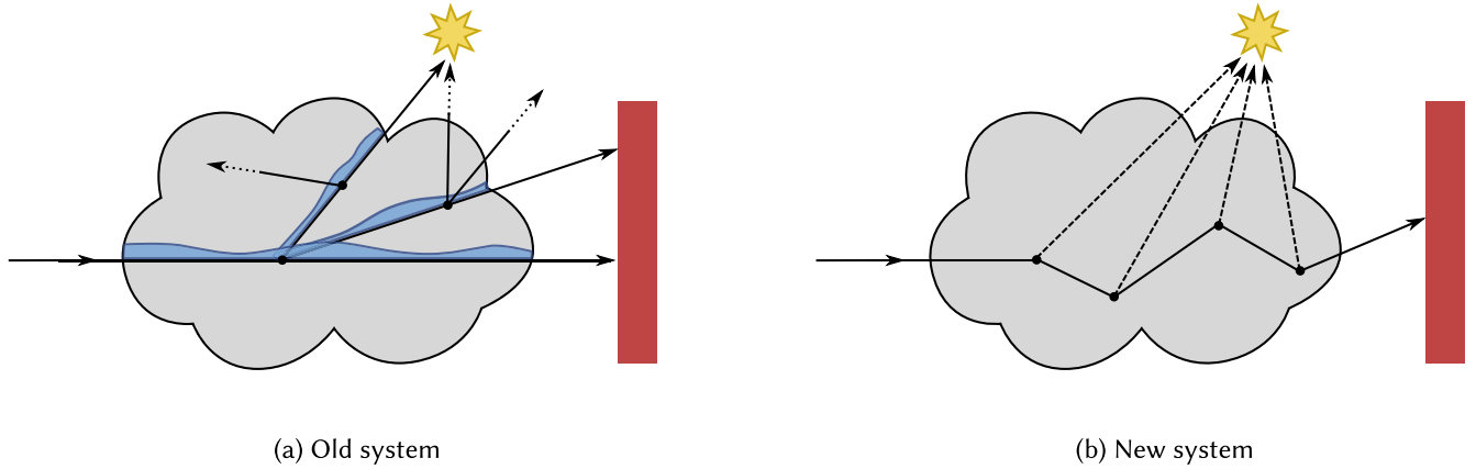
Fig. 11. In our old volume system (left), before shading a surface hit, a detailed PDF (blue) is built along the ray segment encoding transmittance, extinction, and a fluence estimate generated from the cache points. In-scattering samples are drawn and enqueued into a future ray batch. In our new volume system (right), a ray enters the volume and scatters many times based solely on the local scattering properties of the volume. Shadow rays (dashed) are used in conjunction with next-event estimation to importance-sample direct lighting contribution and enqueued into a future ray batch only after completely exiting the volume.
