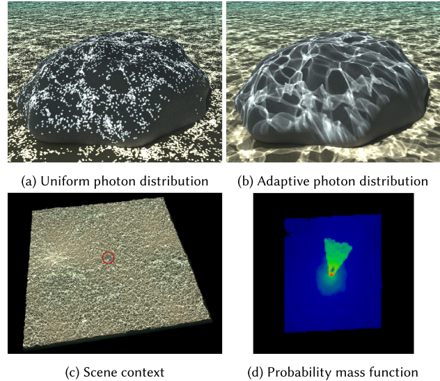
Fig. 6. An example of adaptive photon distribution. (a) and (b) show a close-up of a small rock in a large environment rendered using the same number of photons without and with adaptive photon distribution, respectively. The context of the close-up is shown in (c) with a red circle around the rock, and the probability mass function used for adaptive photon distribution is shown in (d) with the square water surface, camera frustum, region around the camera, rock, and area behind the rock all clearly visible.
