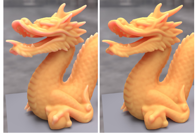
Fig. 9. The Stanford dragon rendered with IOR 1 in (a) shows overly bright thin edges due to the lack of internal reflection. It can be fixed by using a more reasonable IOR value, in this case 1.4 in (b). Dragon model courtesy of the Stanford Computer Graphics Laboratory.
