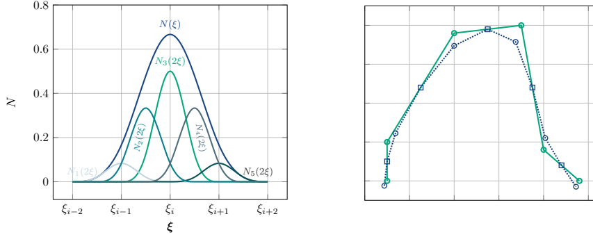
FIG. 3. Left: Refinement of one-dimensional (1D) cubic B-spline ( N(\xi) ). Right: A subdivision applied to the 1D coarse-level control polygon (green) results in refined control polygon (blue). (Color available online only.)
